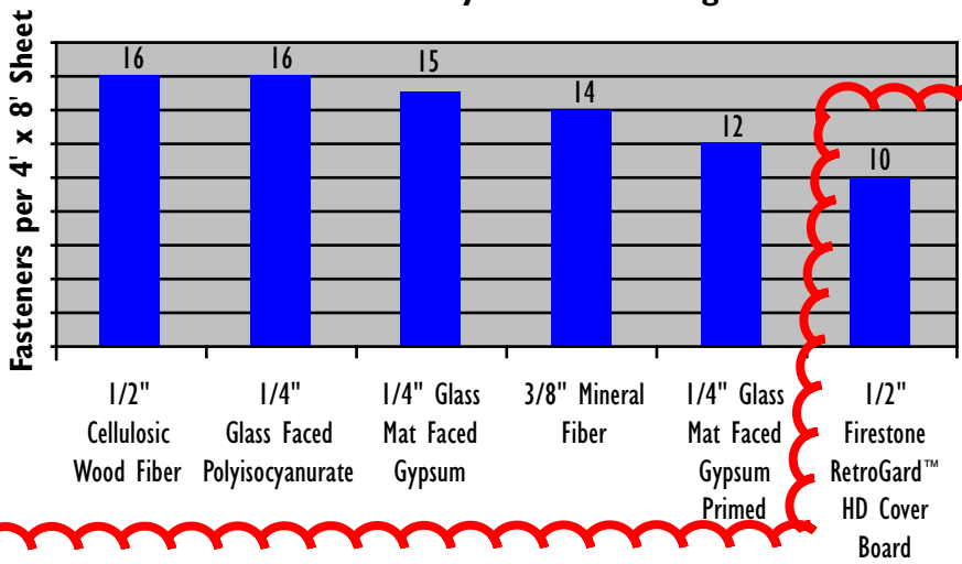
Fastener Density for I-90 Rating
