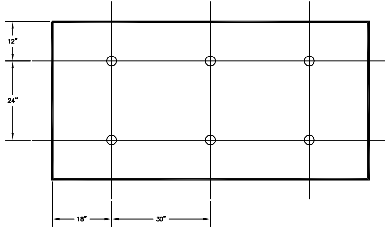
(6 FAST. PER 4' x 8' BOARD)
