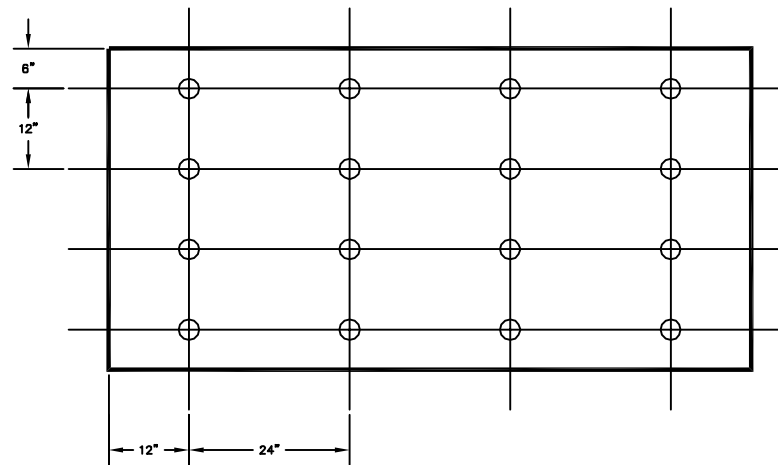
(16 FAST. PER 4' x 8' BOARD)
