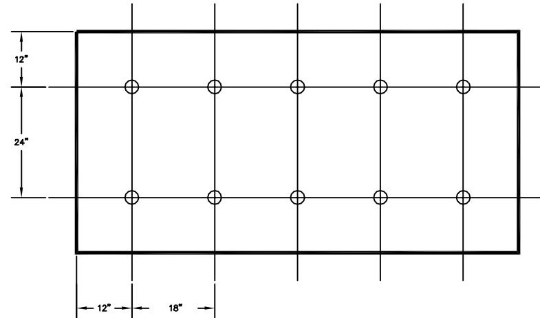
(10 FAST. PER 4' x 8' BOARD)
